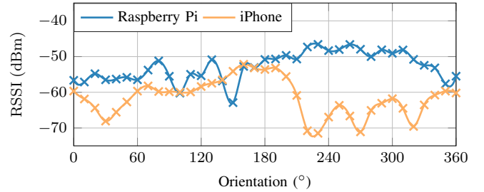
Fig. 1: Interpolated antenna radiation patterns (RSSI) of Raspberry Pi and iPhone 6.
