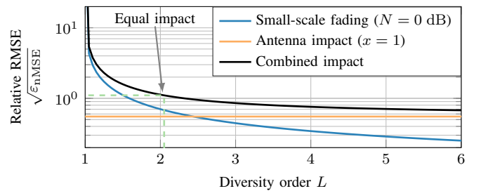
Fig. 5: Relative RMSE of ML distance estimate based on (8) - (12) with \sigma_h = 1 , \sigma_N = 4 dB and \alpha = 2 .
