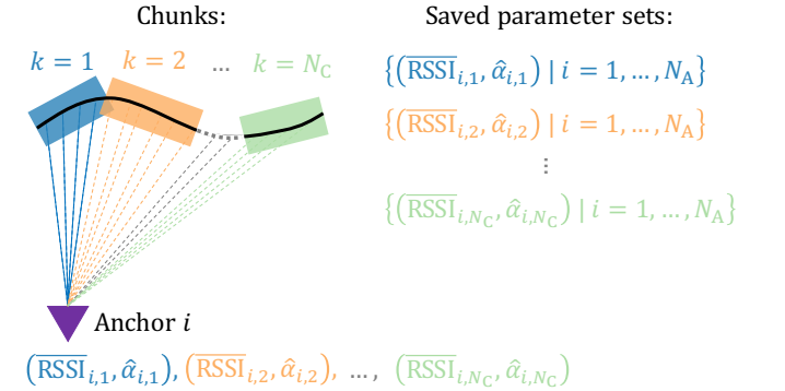
Fig. 6: Schematic illustration of a MRM calibration walk with arbitrary but known true path (black) that is separated into N_C chunks. For simplicity only anchor i is shown.
